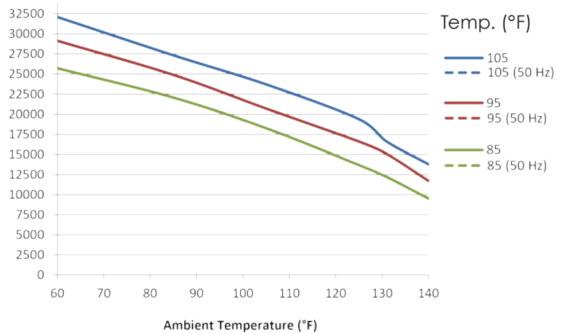
HC20C 240V (60 Hz)
