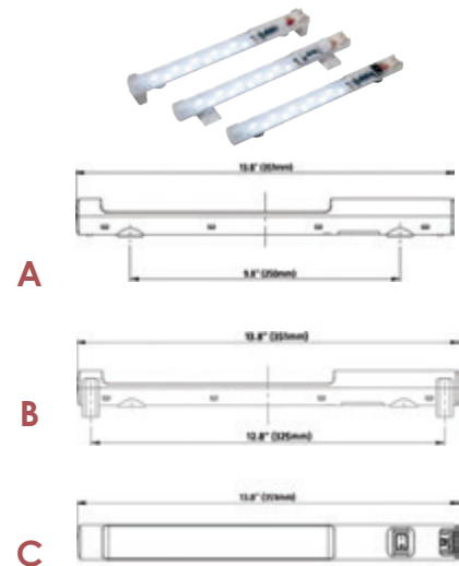
Dimensioned Drawings.
