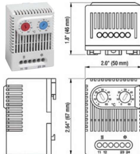
Dimentioned Drawings.
