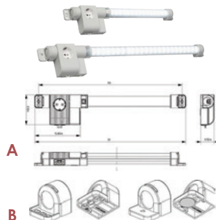
Dimentioned Drawings.
