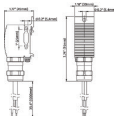
Dimentioned Drawing.
