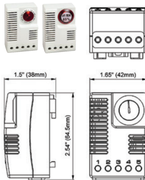
Dimensioned Drawings.
