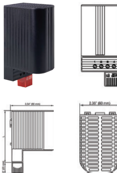
Dimensioned Drawings.
