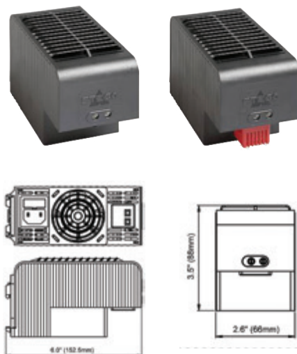
Dimensioned Drawings CS 032.
