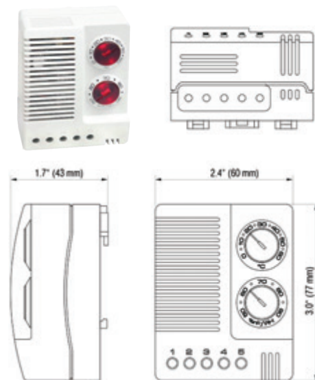
Dimentioned Drawings.
