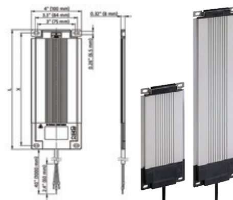
Dimensioned Drawings.
