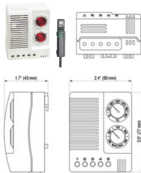
Dimentioned Drawings.
