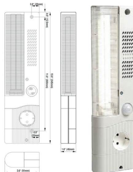
Dimentioned Drawings.
