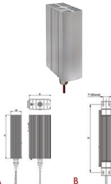
Dimensioned Drawing. A) with DIN clip.
