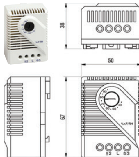
Dimentioned Drawings.
