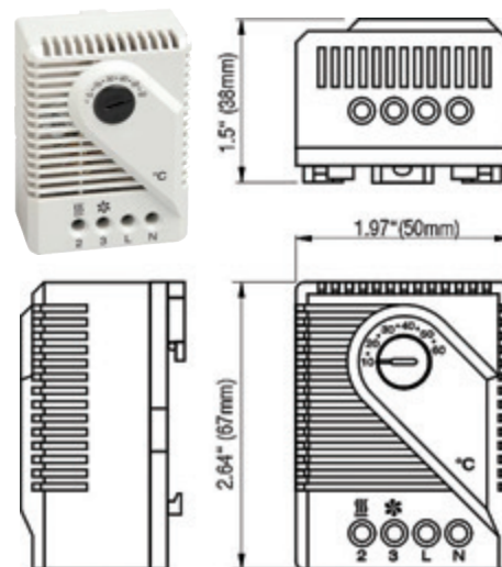
Dimentioned Drawings.
