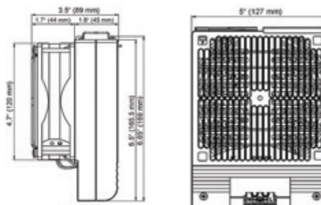
Dimensioned Drawings.
