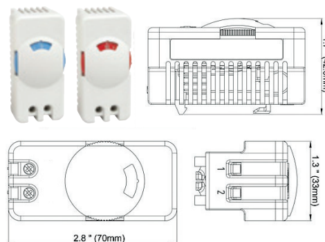
Dimensioned Drawings.
