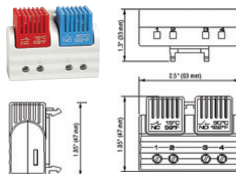
Dimentioned Drawings.
