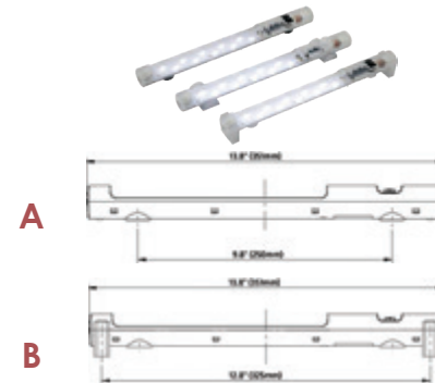
Dimensioned Drawings.
