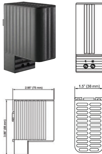
Dimensioned Drawings.
