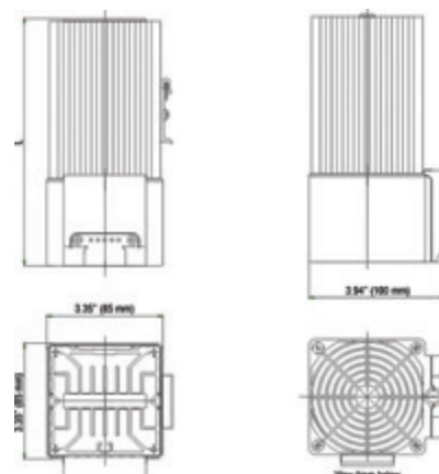
Dimentioned Drawings.
