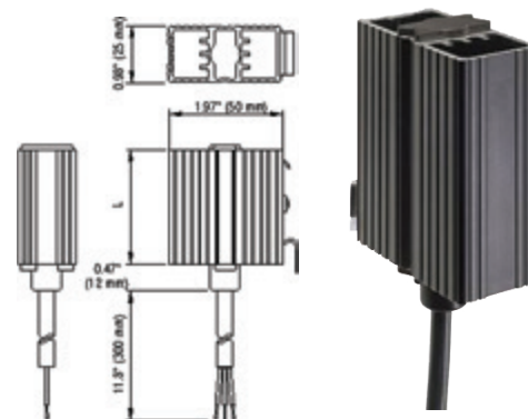
Dimensioned Drawings.
