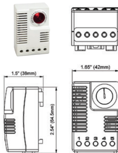
Dimentioned Drawings.
