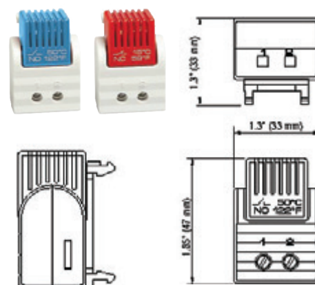
Dimensioned Drawings.
