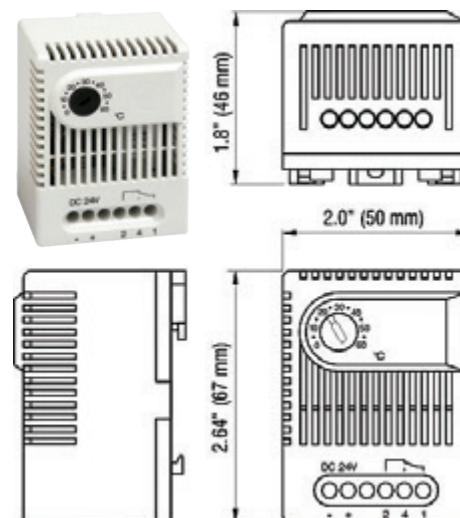
Dimensioned Drawings.
