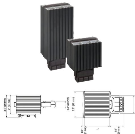
Dimensioned Drawings.
