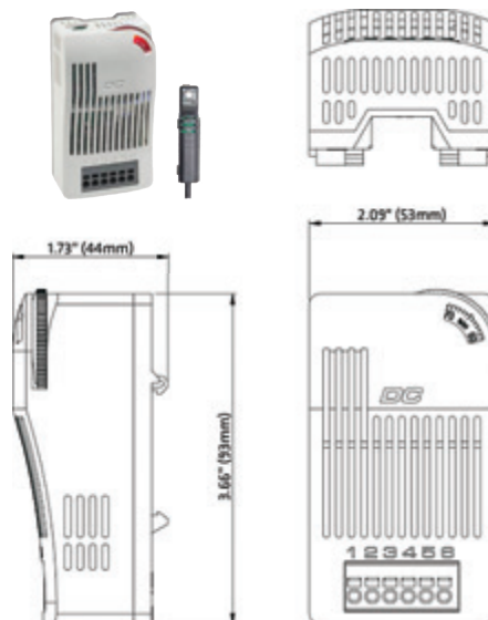
Dimensioned Drawings.
