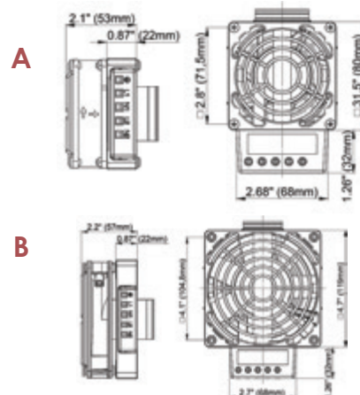
Dimensioned Drawings. A) 100 W/ 150 W Heater. B) 200 W/ 300 W/ 400 W Heater.
