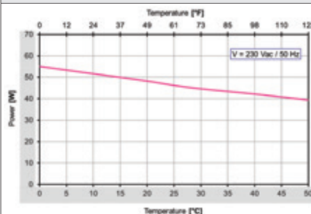
Power-Temperature
