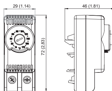
Technical drawing mm (in)
