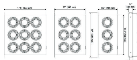
Dimentioned Drawings.
