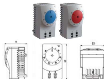
Dimensioned Drawings
