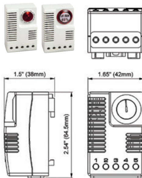
Dimensioned Drawings.
