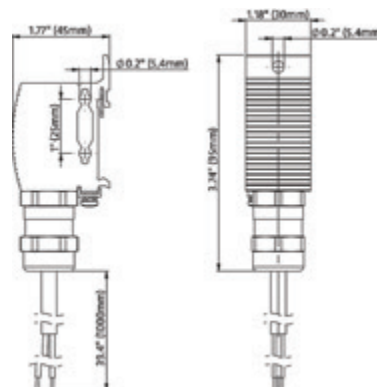
Dimentioned Drawing.
