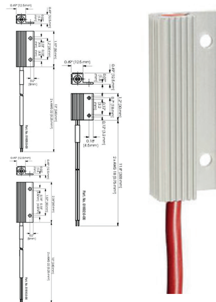
Dimensioned Drawings.
