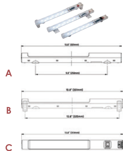
Dimentioned Drawings.
