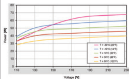
Power-Temperature
