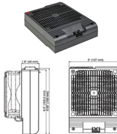
Dimensioned Drawings.
