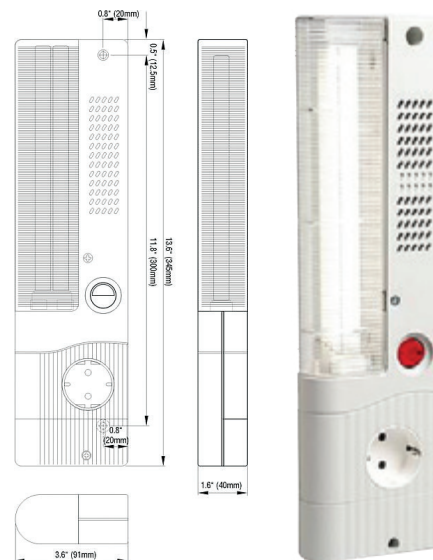
Dimensioned Drawings.
