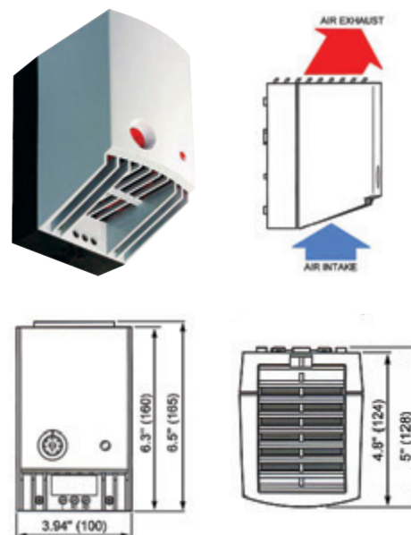
Dimensioned Drawing.
