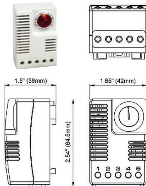
Dimensioned Drawings.
