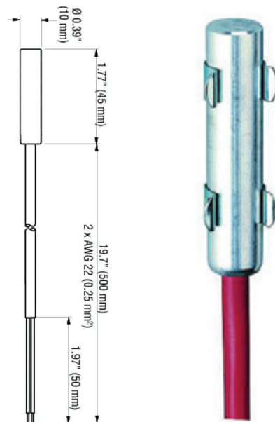
Dimensioned Drawing.
