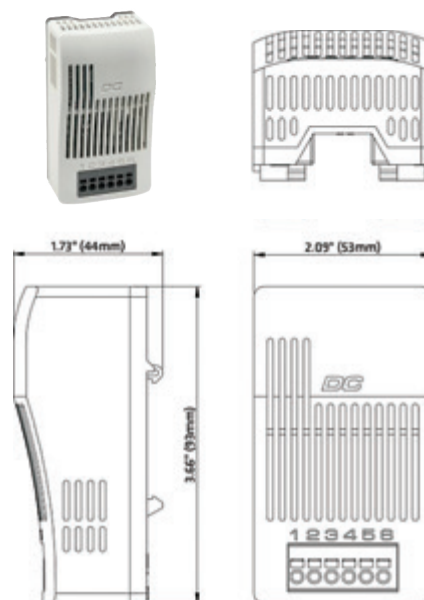
Dimentioned Drawings.
