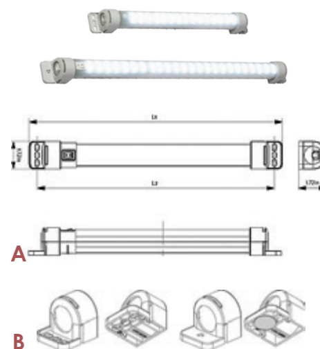
Dimensioned Drawings.
