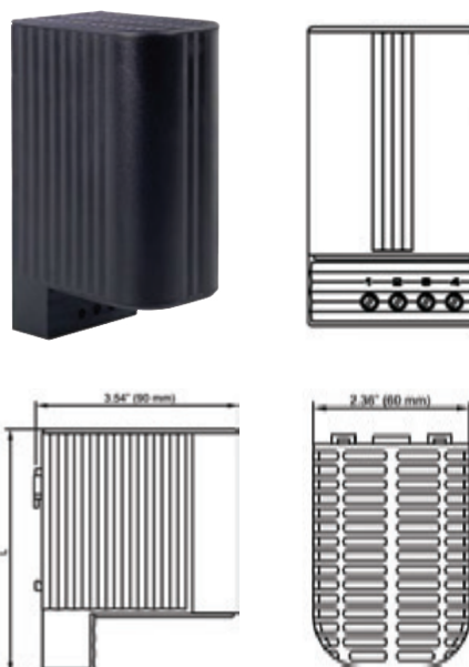
Dimensioned Drawings.
