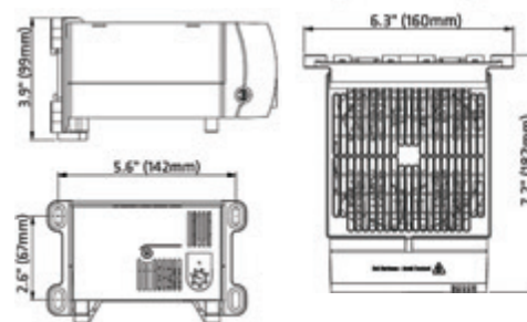
Dimentioned Drawings.
