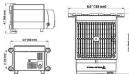
Dimensioned Drawings.
