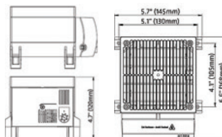
Dimentioned Drawings.
