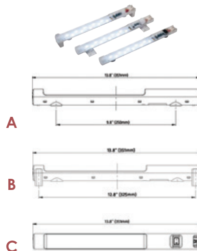
Dimentioned Drawings.
