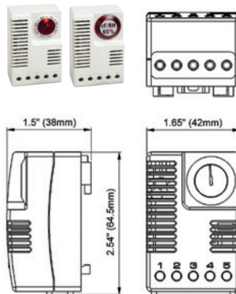
Dimensioned Drawings.
