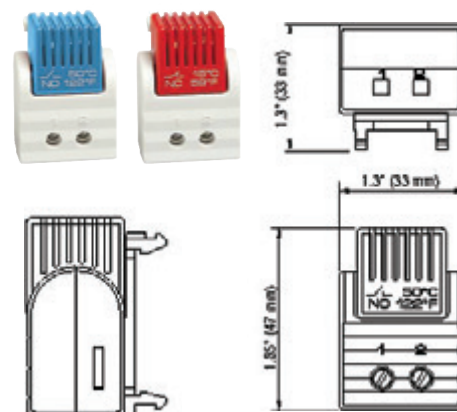
Dimensioned Drawings.
