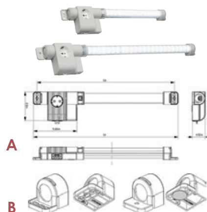
Dimentioned Drawings.
