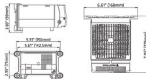
Dimensioned Drawings.
