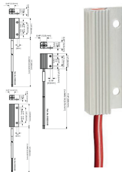
Dimensioned Drawings.
