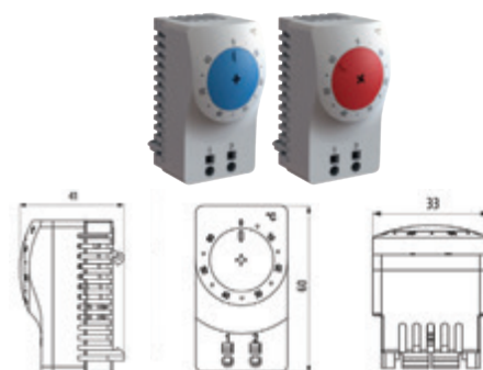
Dimentioned Drawings
