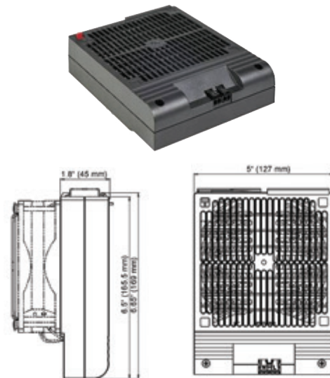
Dimensioned Drawings.
