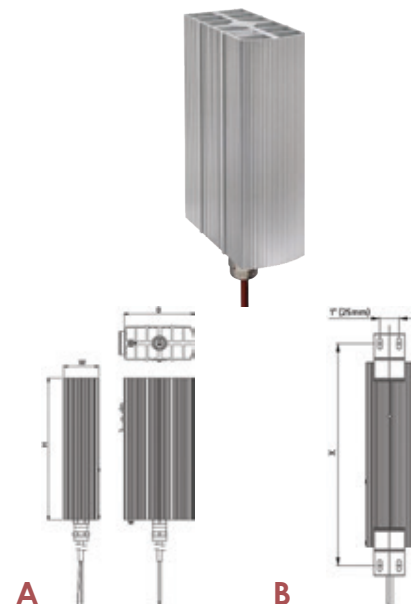
Dimensioned Drawing. A) with DIN clip.
