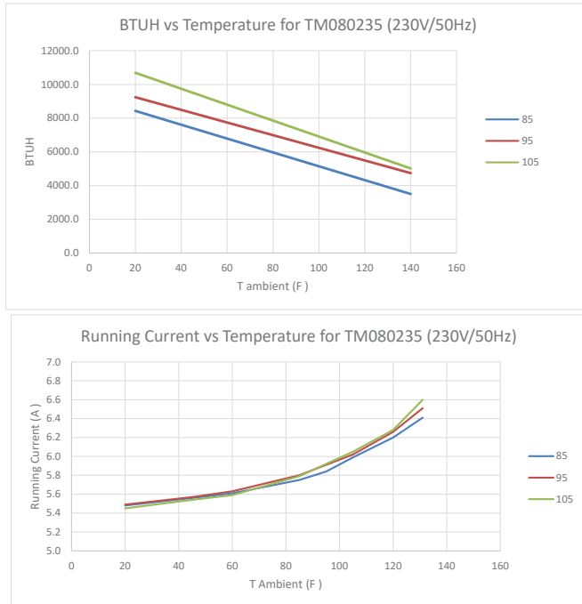
TM081 60 Hz unit test results running on 50 Hz power source
