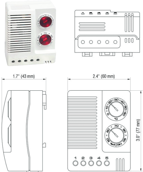
Dimensioned Drawings.
