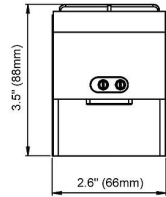
Dimensioned Drawings CS 032.
