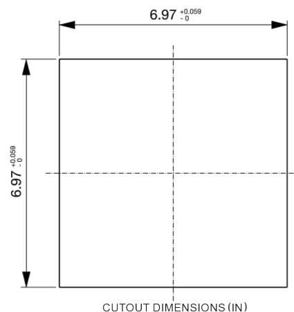
CUTOUT DIMENSIONS (IN)
