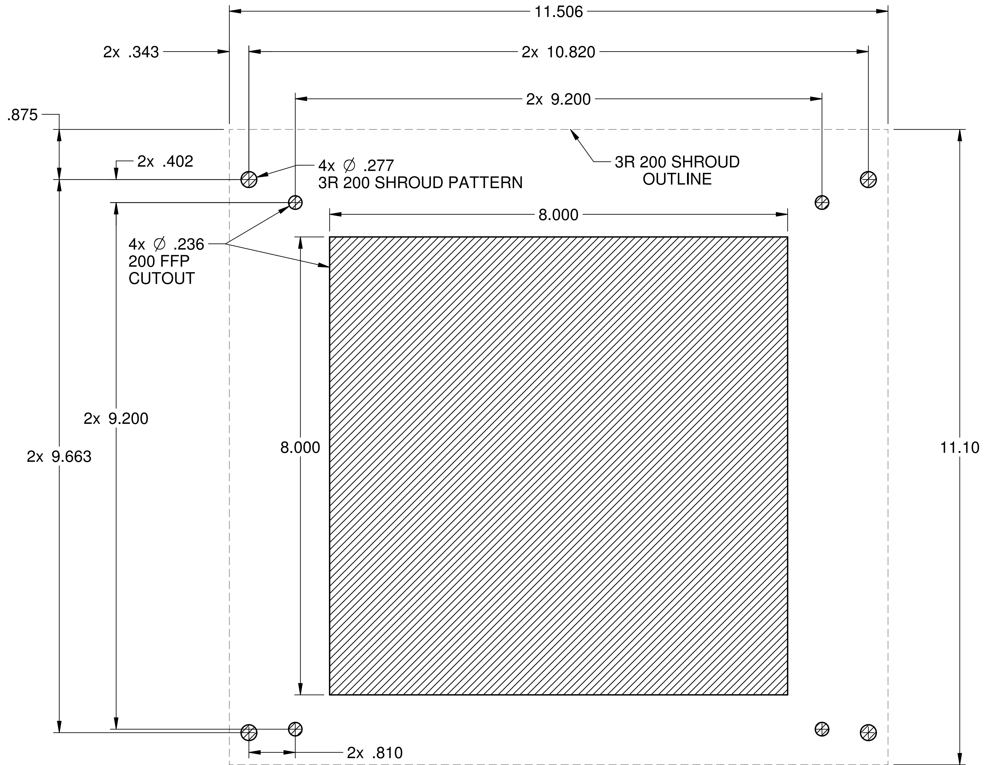
CUTOUT TEMPLATE 200 FFP WITH 3R 200 RAIN SHROUD (VERIFY PRINT ACCURACY BEFORE USE)
