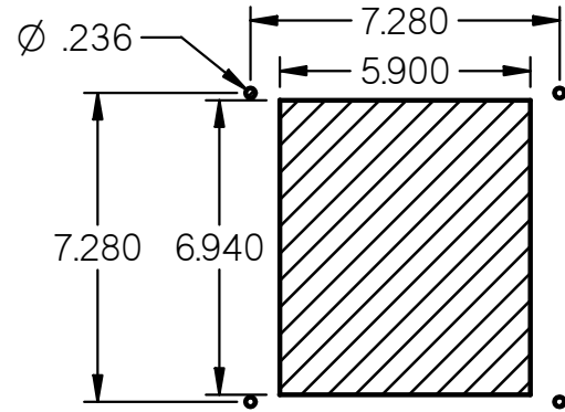
CUTOUT DRAWING 1:5
